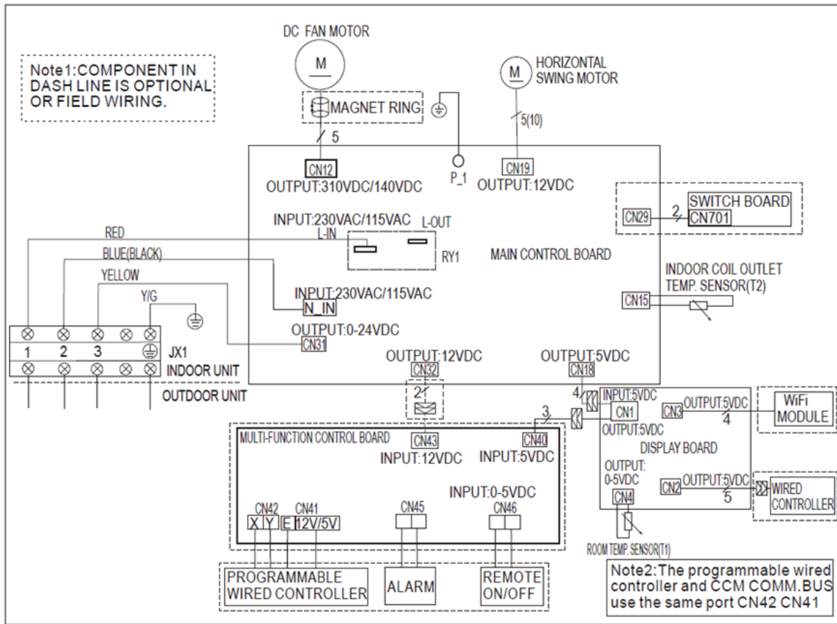
Fig. 7 — Wiring Diagram Sizes 12K (115V) and 6K - 12K (208/230V)
