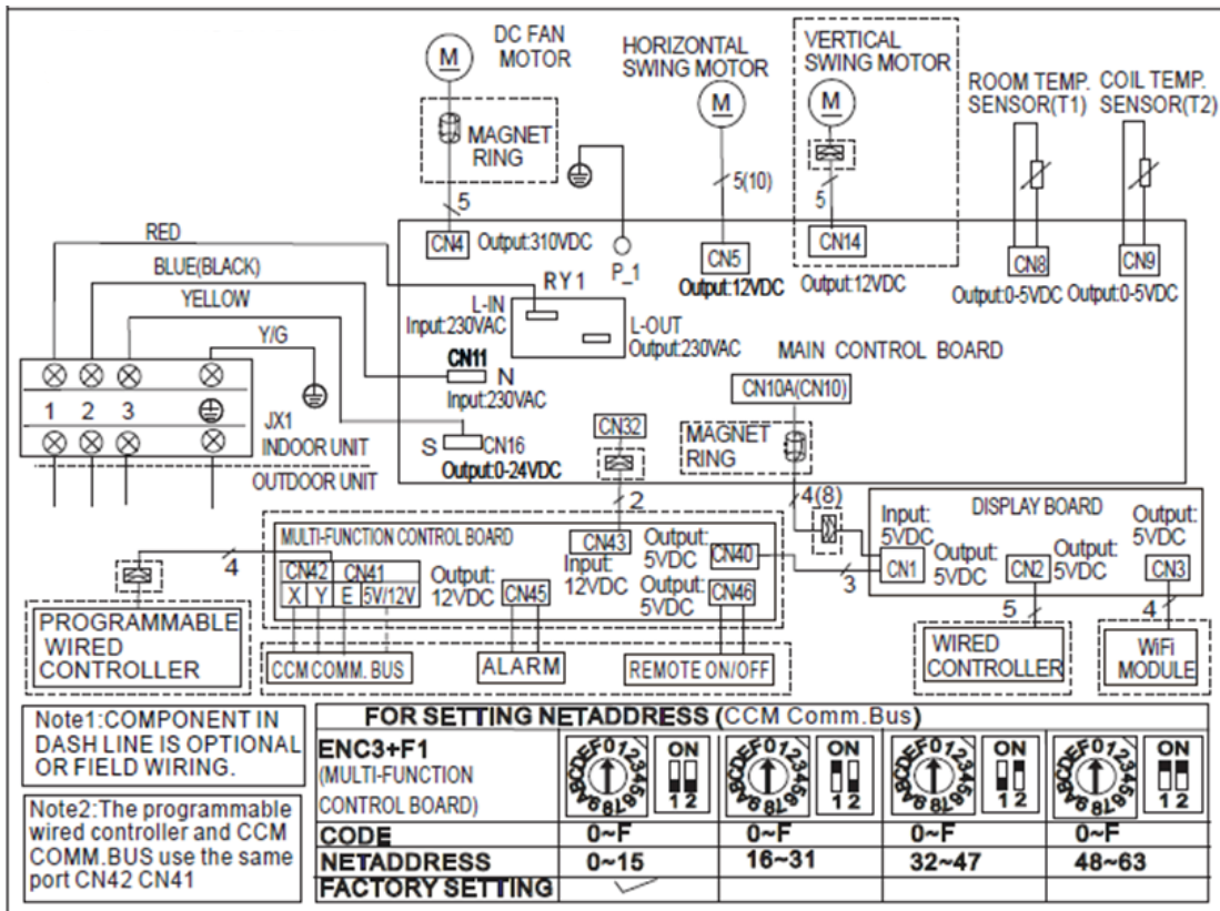
Fig. 8 — Wiring Diagram Sizes 18K - 36K (208/230V)
